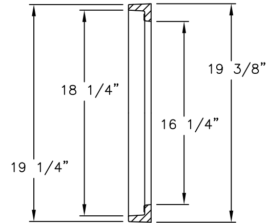
FRAME SECTION
