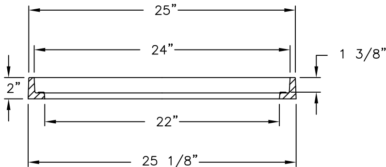
FRAME SECTION
